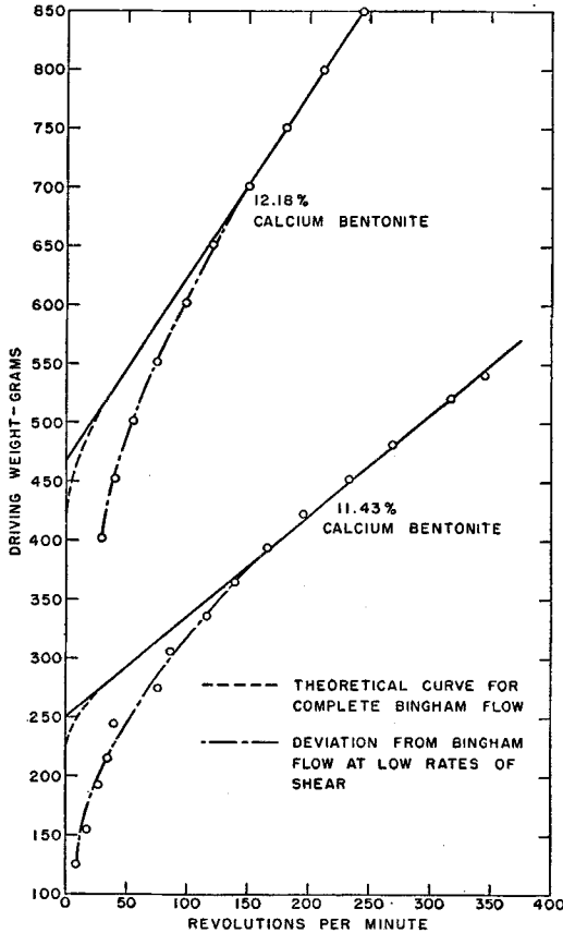
FIGURE 1.—Bingham flow curves obtained with the modified Storrer viscometer.
