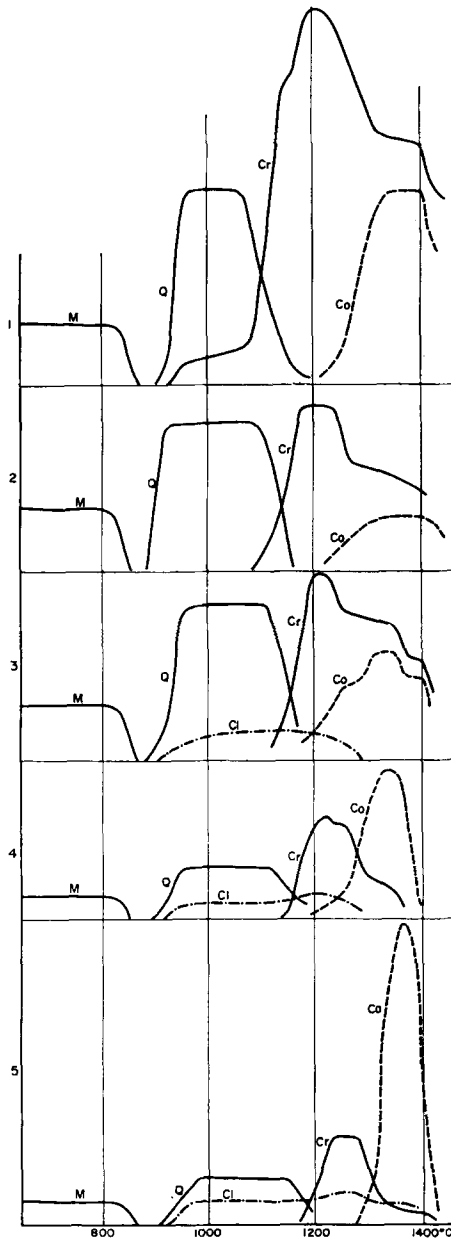
FIGURE 8. — Intensities of diffraction lines of high-temperature phases in Cheto montmorillonite: Mg-clay (1); Mg-clay and 100 meq (2), 200 meq (3), 500 meq (4), 1000 meq (5), of MgCl_2 added. Same notations as in Figure 2. Enstatite, Cl.
