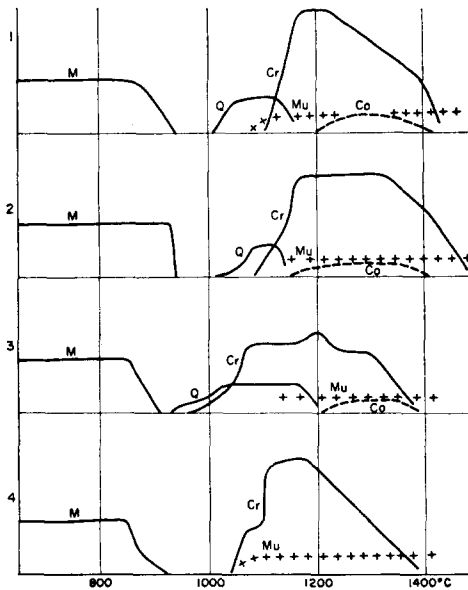
FIGURE 9.— Intensities of diffraction lines of high-temperature phases in Montmorillonite: untreated (1); exchanged with H (2), Li (3), Na (4). Same notations as in Figure 2.
