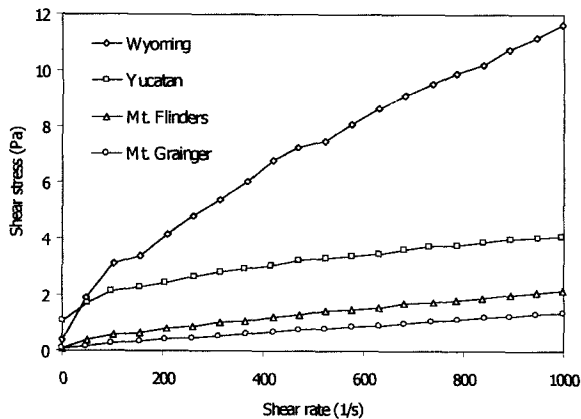
Figure 1. Flow curves of 3% w/v suspensions of Na-saturated clays at pH 7.
