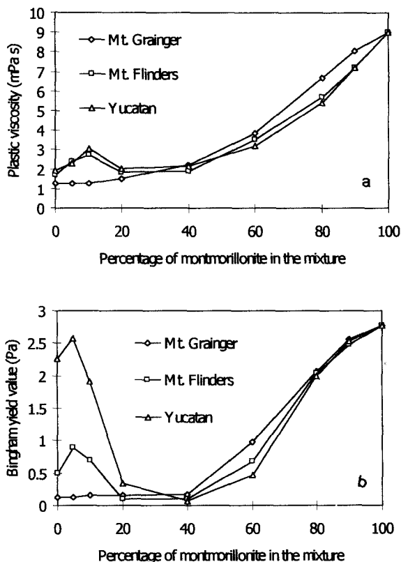
Figure 2. Effect of montmorillonite concentration on plastic viscosity (a) and Bingham yield value (b) of mixed suspensions of Na-saturated palygorskite and montmorillonite at a total clay concentration of 3% w/v and pH 7.
