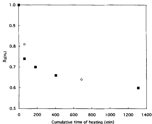
Figure 2. The fraction of hydrogen, X_s(\text{H}_2) , remaining in the sample plotted against the cumulative time of heating (at 250°C) for halloysite 1, experiment MHD-1945 (■) and for halloysite 2, experiment MHD-1950 (○). The rate of H loss (evolved as water) decreases with time. Despite different total water contents (see footnote to Table 1), between 36–40% of the structural hydrogen of the OH group (reported as water) is lost from both samples after \sim 685 min of heating at 250°C in vacuo .
