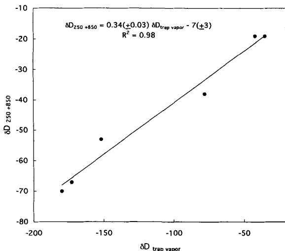
Figure 3. The \delta D value for structural hydrogen of the OH group in halloysite ( \delta D_{250+850} ) after exchange with water vapor at 22°C plotted against the \delta D value of the final exchanged water vapor ( i.e. , trap vapor, see text). The solid line represents a linear regression fitted through the data. The equation for the regression is shown.
