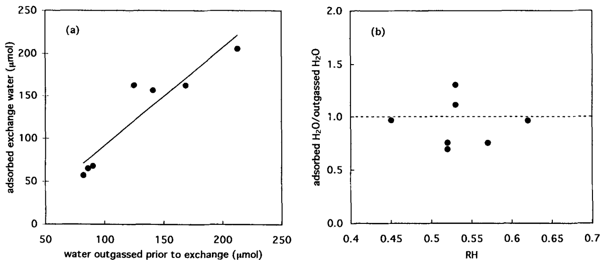
Figure 1. (a) The calculated amount of water adsorbed on halloysite during exchange plotted against water removed during the initial outgassing at 100°C prior to exchange. The slope of the linear regression (solid line) is 1.15, the intercept is -24 , and the R^2 value is 0.87. (b) The ratio of the amount of water adsorbed on halloysite during exchange relative to water removed during outgassing at 100°C prior to exchange plotted against the "relative humidity" in the sample chamber. The dotted line represents a reference ratio of unity.
