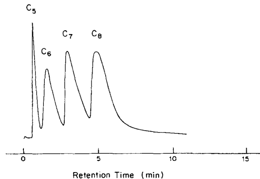
Figure 4. Chromatographic separation of C_5 – C_8 hydrocarbons by a TPP-montmorillonite column: column: 3 ft \times \frac{1}{8} in. o.d. carrier gas He: at 45 ml/min column temperature: 90°C hold 1 min, then to 170°C at 20°C/min.
