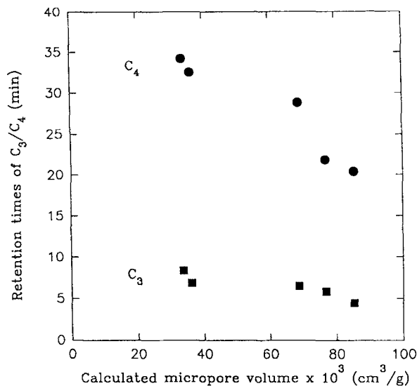
Figure 3. Correlation between the retention times of hydrocarbons ( C_3/C_4 ) and the calculated micropore volume of the organo-clays.
