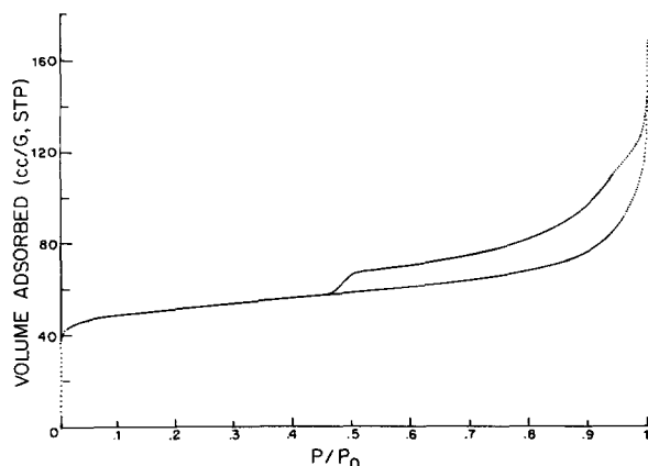
Figure 1. Nitrogen adsorption and desorption isotherms of the organo-montmorillonite MMDA-M.
