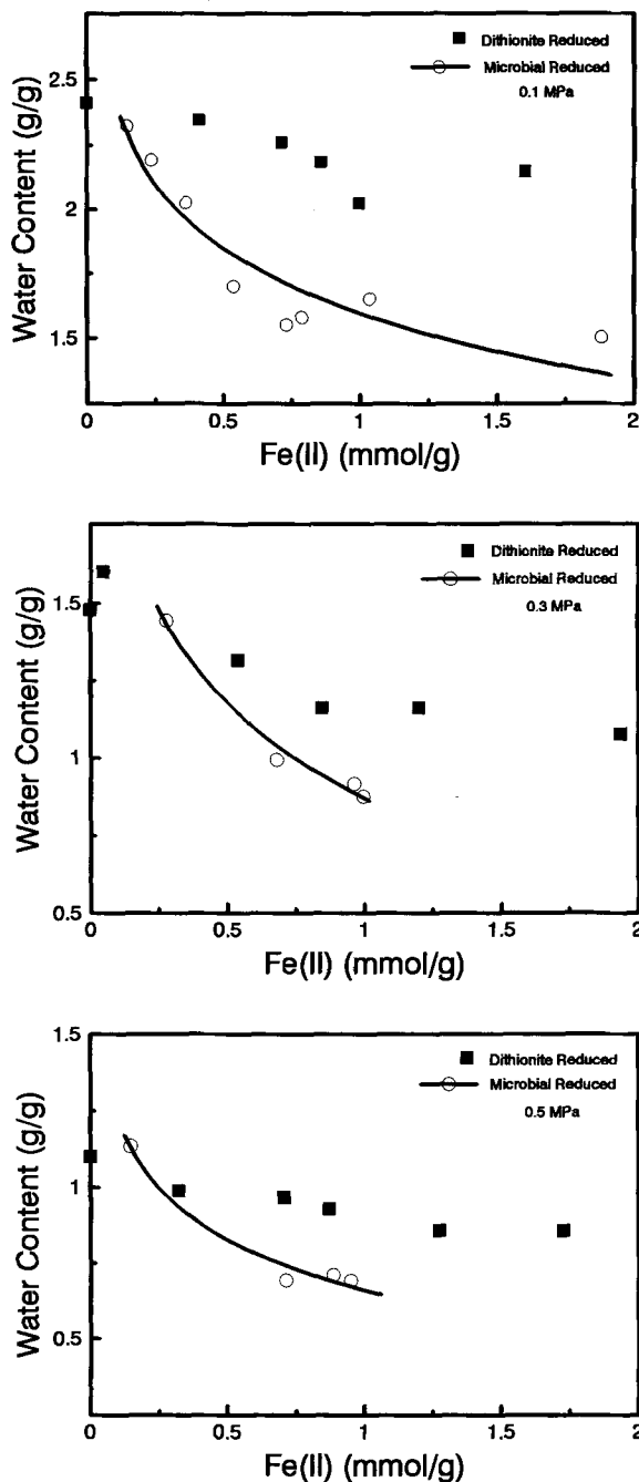
Figure 1. Effect of structural Fe(II) on the water content ( m_w/m_c ) of SWa-1 reduced by combined Pseudomonas inoculum suspensions (PIS and SIS) and dithionite at a) 0.1 MPa, b) 0.3 MPa, and c) 0.5 MPa applied pressure. Solid lines represent best fits; data for dithionite from Lear and Stucki, 1989.
