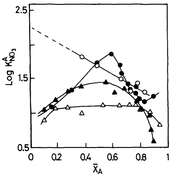
Figure 1. Kielland plot for OH^- or F^-/NO_3^- exchange on hydrotalcite. OH^-/NO_3^- exchange: ● by Miyata, ○ recalculated, F^-/NO_3^- exchange: ▲ by Miyata, △ recalculated.
