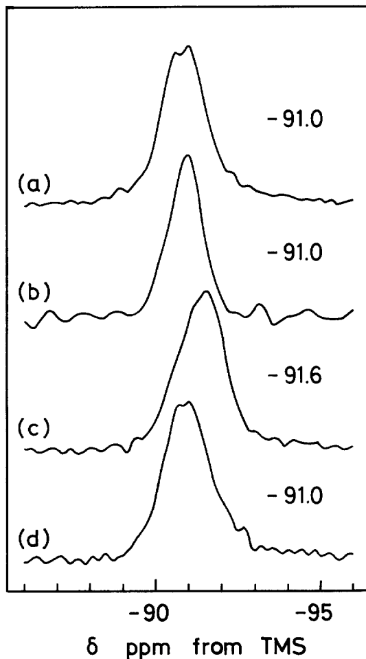
Figure 5. 29 Si nuclear magnetic resonance spectra with cross polarization and magic angle spinning of (a) raw kaolinite, (b) kaolinite-N-methylformamide intercalation compound, (c) kaolinite-acrylamide intercalation compound, and (d) kaolinite-acrylamide intercalation compound heated at 300°C for 1 hr.
