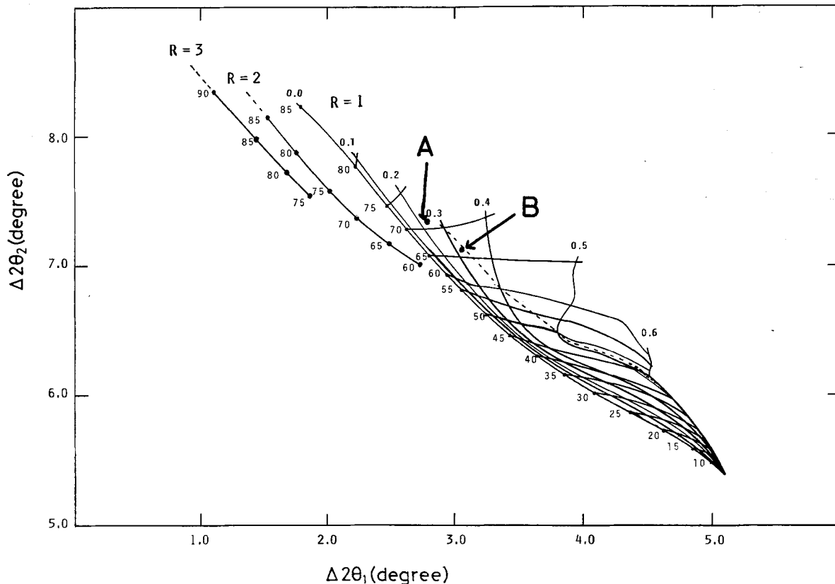
Figure 4. Diagram for quantification of mica/glycolated-smectite interstratifications. Dotted line indicates random structure ( R=0 ). A: Two Medicine, Wyoming. B: Kinnkulle A-2, Sweden.
