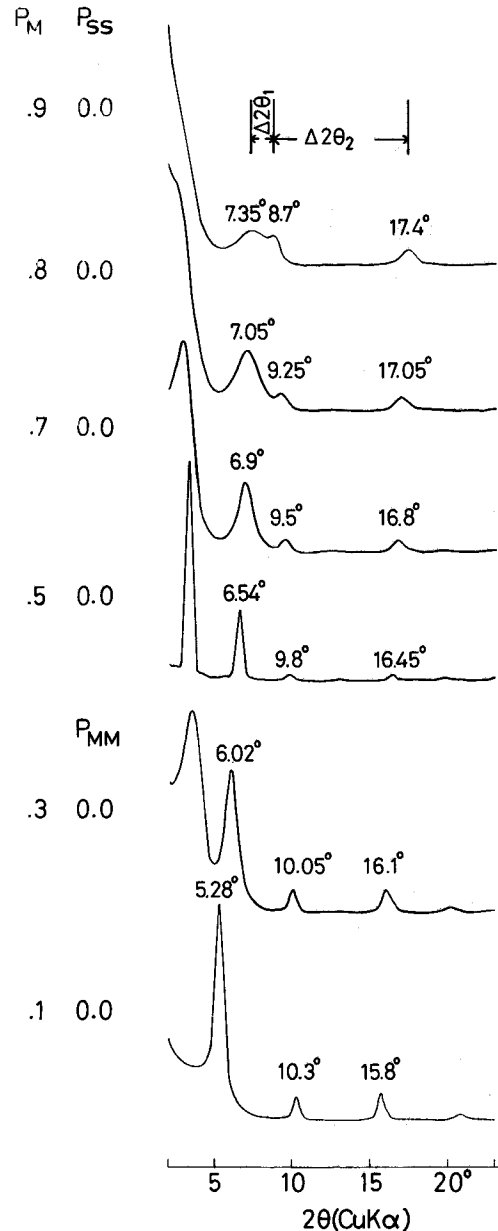
Figure 2. Calculated X-ray powder diffraction patterns for various interstratified structures. P_M is probability of existence of mica layer. P_{SS} is probability that a smectite layer succeeds a smectite layer given that the first layer is a smectite layer. P_{MM} is similarly defined.
