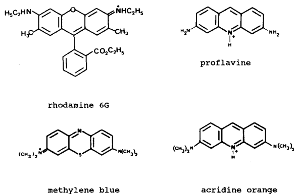
Figure 1. Structural formulae of the dye molecules.
