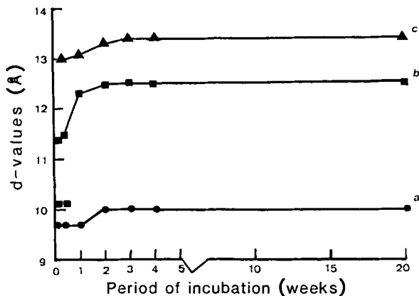
Figure 2. Reexpansion (Å) of n-alkylammonium ion-exchanged samples following Li-saturation and heat treatment as a function of time: (a) sample SAz-1 (●) and (b) sample SWy-1 (■) exchanged with hexylammonium ions; (c) sample B 18/4 (▲) exchanged with dodecylammonium ions. Notice the two d(001) reflections (first four data points) observed for sample SWy-1 in 24 and 48 hr of incubation which indicate the different rates of exchange of the organic cations in the interlayers.
