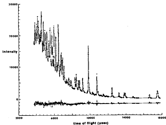
Figure 1. Neutron time-of-flight data for deuterated boehmite at 18°C. Upper plot: Observed data shown by + symbols; calculated data for space group Cmc21 shown by solid line. Lower plot shows observed minus calculated. Regions excluded from refinement shown by absence of observed data points. Range is from 3660 \mu\text{sec} (0.49 Å) to 18,000 \mu\text{sec} (2.41 Å) and includes 350 possible Bragg reflections. Neutron time of flight is linearly proportional to d-value with a constant of proportionality of 7470 \mu\text{sec}/\text{Å} for the instrument used in this study.
