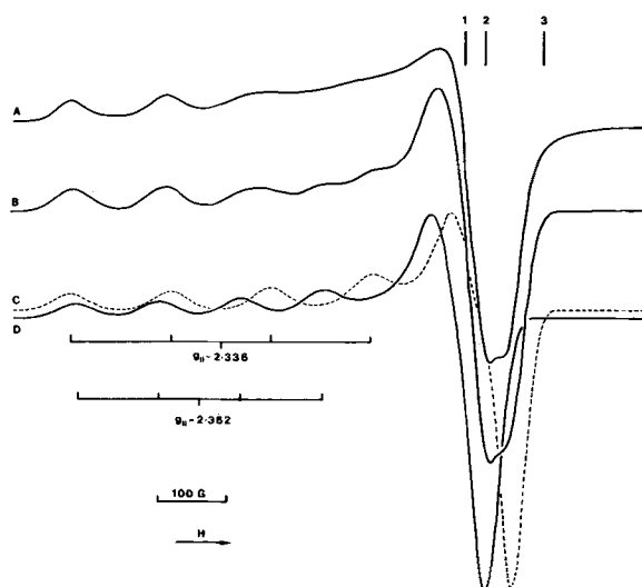
Figure 7. Actual (A) and simulated (B) electron spin resonance spectrum at 22°C of \text{Cu}^{2+} adsorbed on sample SA 1.10 at pH 6.0. Two computer-generated spectra of \text{Cu}^{2+} , (C) and (D), were used to construct the simulated (B) spectrum. The numbered vertical lines represent the g_{\perp} resonance positions at 2.075 (1) and 2.056 (2), and the free electron field position at 2.0023 (3).
