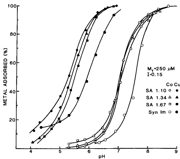
Figure 2. Adsorption of \text{Cu}^{2+} and \text{Co}^{2+} by synthetic allophane and imogolite as a function of pH from a 0.05 M \text{Ca}(\text{NO}_3)_2 solution containing 2.5 \times 10^{-4} M metal.
