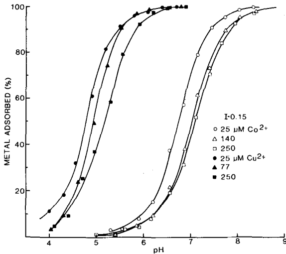
Figure 3. Adsorption of \text{Cu}^{2+} and \text{Co}^{2+} by Te Akatea allophanic clay as a function of pH and metal concentration from a 0.05 M \text{Ca}(\text{NO}_3)_2 solution.
