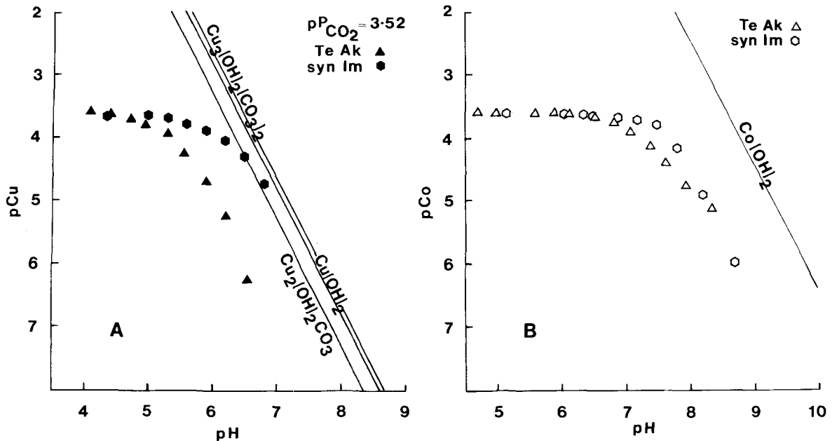
Figure 4. Solubility of Cu and Co (plotted as \text{pM} = -\log(\text{M}^{2+}) ) after 24-hr equilibration of Te Akatea clay and synthetic imogolite in (A) 2.5 \times 10^{-4} M Cu in 0.05 M \text{Ca}(\text{NO}_3)_2 , and (B) 2.5 \times 10^{-4} M Co in 0.05 M \text{Ca}(\text{NO}_3)_2 . Solubility lines for copper hydroxide, malachite, and azurite were determined from the data of Lindsay (1979), and cobalt hydroxide from those of Baes and Mesmer (1976), assuming atmospheric partial pressure of \text{CO}_2 ( -\log P_{\text{CO}_2} = 3.52 ).
