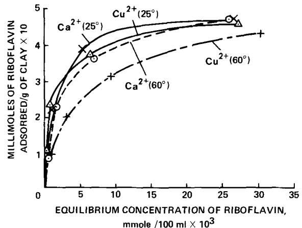
Figure 3. Adsorption isotherms of riboflavin on \text{Cu}^{2+} - and \text{Ca}^{2+} -smectite at two temperatures.
