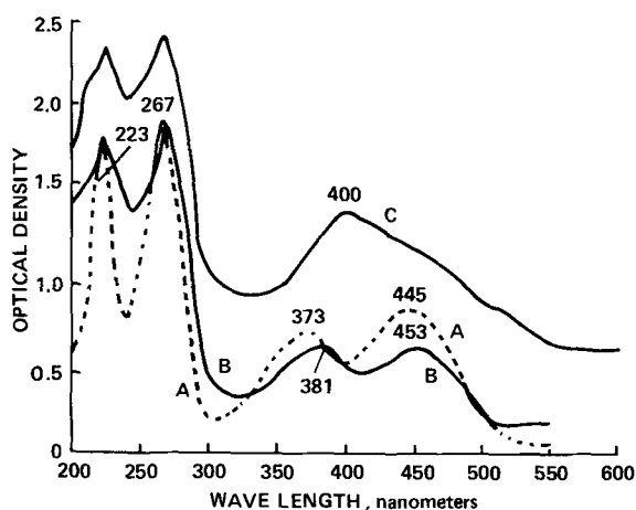
Figure 4. (A) UV-visible spectra of riboflavin in H 2 O (0.0025 mmole/100 ml); (B) complexed with Cu 2+ -smectite (film on quartz plate in H 2 O); (c) sample B heated to 75°C and covered with mineral oil.
