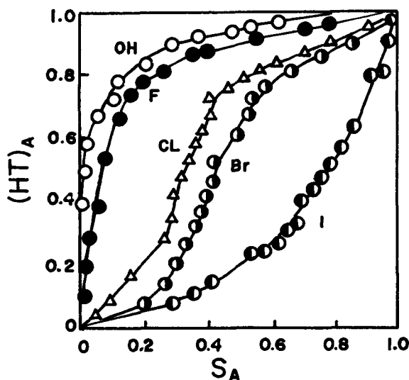
Figure 1. Ion-exchange isotherms for the HT-NO 3 -OH - (○), HT-NO 3 -F - (●), HT-NO 3 -Cl - (△), HT-NO 3 -Br - (◐), and HT-NO 3 -I - (◑) systems at 0.1 total normality and 25°C.
