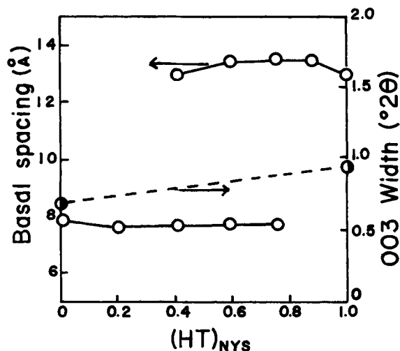
Figure 11. Basal spacing (○) and width of the 003 reflection (●) for the HT-Cl-NYS 2- system as a function of HT composition.
