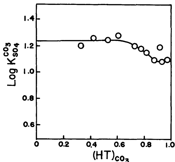
Figure 9. Selectivity coefficient for the HT-SO 4 -CO 3 2- system as a function of HT composition.
