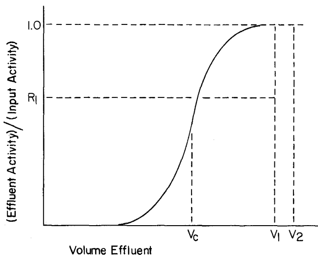
FIGURE 1.—Elution chromatogram.
