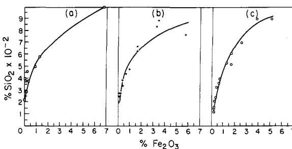
Figure 2. Percentages of \text{SiO}_2 extracted in a modified dithionite (CDB) treatment with respect to extracted \text{Fe}_2\text{O}_3 in samples a, b, and c.
