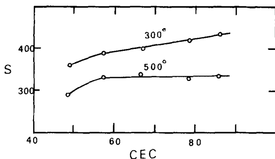
Figure 6. Surface area S , in m^2/g , of reduced charge, Zr-montmorillonites after heating at 300° and 500°C.
