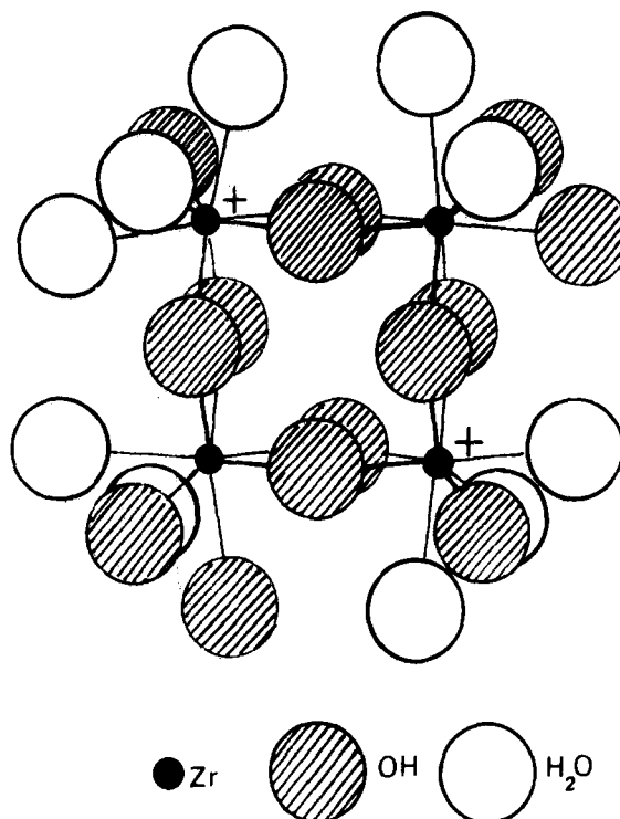
Figure 7. Probable form of the [Zr_4(OH)_{14}(H_2O)_{10}]^{2+} complexes.
