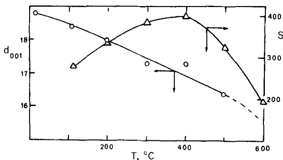
Figure 1. Basal spacings, d(001) , in Å and surface areas, S , in m^2/g , of zirconium montmorillonites heated 20 hr at temperatures T , ^{\circ}C .
