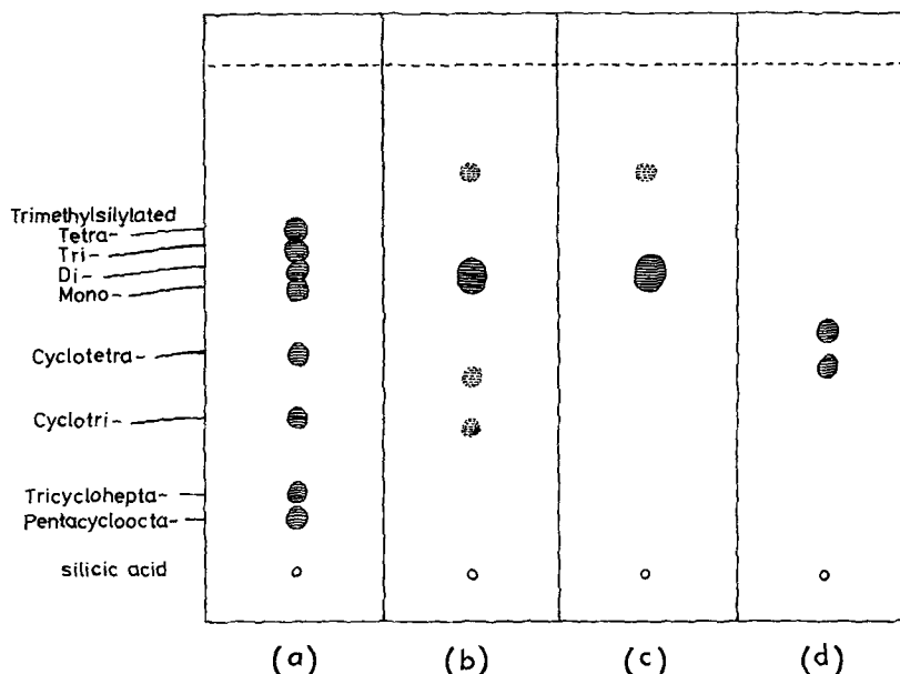
Figure 2. Thin-layer chromatograms of the trimethylsilylated products: (a) data from Hoebbel and Wieker (1974) on \text{Al}_2\text{O}_3 - \text{SiO}_2 plate; (b) soluble product (A) on \text{Al}_2\text{O}_3 - \text{SiO}_2 plate; (c) soluble product (B) on \text{Al}_2\text{O}_3 - \text{SiO}_2 plate; (d) soluble product (A) on \text{SiO}_2 plate.
