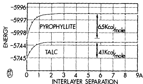
Fig. 1. A plot of the electrostatic energy (in e^2/\text{\AA} ) of pyrophyllite and talc vs the increase in the interlayer distance. The 0. \text{\AA} separation corresponds to the normal crystal structure and the energy difference between this and the expanded structures ( > 3 \text{\AA} ) is an estimate of the energy of the ionic interlayer bonding.
