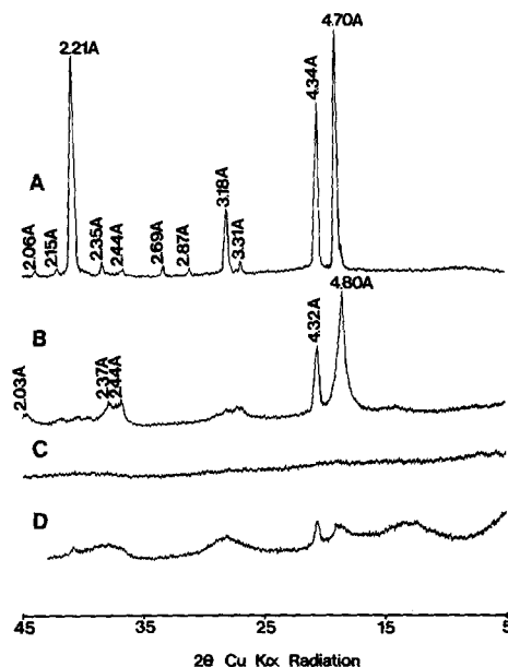
Fig. 1. X-ray diffraction patterns of hydrolytic reaction products of Al at the initial OH/Al molar ratio of 3 and (A) Al concentration of 1 \cdot 10 \times 10^{-3} M in the absence of citric acid collected after 40 day ageing at room temperature, (B) Al concentration of 1 \cdot 10 \times 10^{-3} M in the presence of 10^{-6} M citric acid collected after 40 day ageing at room temperature, (C) Al concentration of 1 \cdot 10 \times 10^{-3} M in the presence of 10^{-4} M citric acid collected after 40 day ageing at room temperature followed by 3 day ageing at 80^\circ\text{C} and (D) Al concentration of 1 \cdot 10 \times 10^{-4} M in the presence of 10^{-6} M citric acid collected after 40 day ageing at room temperature.
