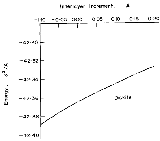
Fig. 2. The variation in the Coulomb energy of dickite as a function of the interlayer separation distance.
