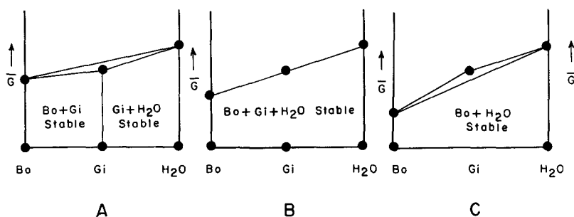
Fig. 3. Schematic molar free energy (chemical potential diagrams) for three conditions. 3A below the reaction curves of Figs. 1 and 2, 3B on the curves, and 3C above the curves. Gi—gibbsite, Bo—boehmite.
