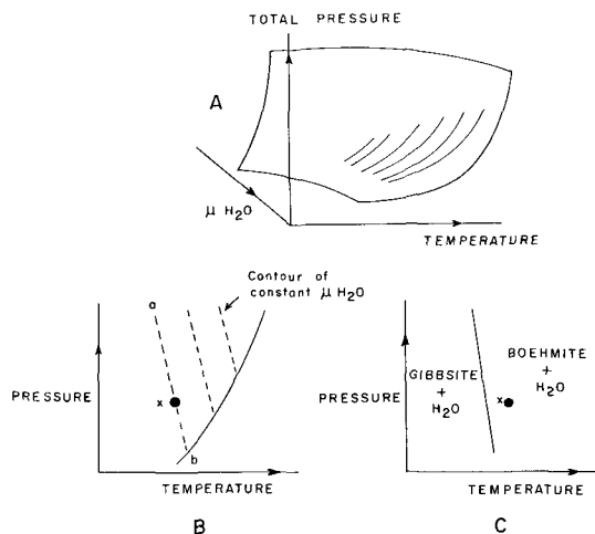
Fig. 2. A diagrammatic representation of the reaction Gibbsite = Boehmite + \text{H}_2\text{O} as a function of three independent variables. 2A is the complete reaction surface. 2B is the reaction surface projected onto the PT plane and contoured for \mu_{\text{H}_2\text{O}} . 2C is the reaction curve at a particular, constant value of \mu_{\text{H}_2\text{O}} . The point labelled x represents the generalized low PT of the earth's surface. The \mu_{\text{H}_2\text{O}} contour a-b is the critical one that passes through x.
