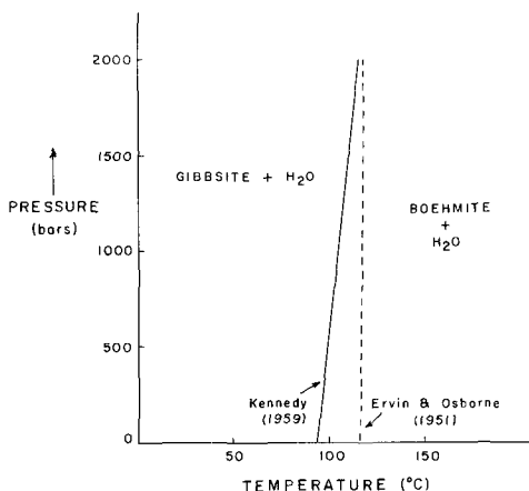
Fig. 1. Two versions of the reaction curve Gibbsite—Boehmite + \text{H}_2\text{O} in a closed system oversaturated with respect to \text{H}_2\text{O} .
