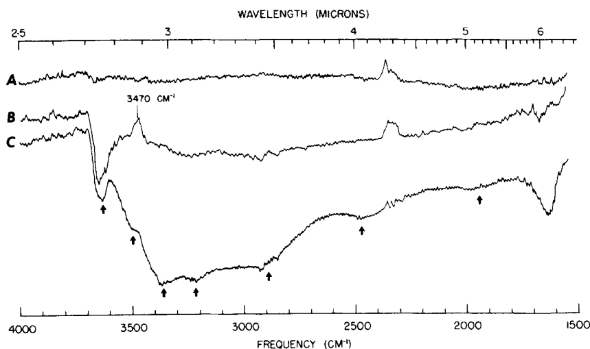
Fig. 1. Differential i.r. spectra of lithium nitrate treated muscovite after hydrogen saturation. A—Matched specimens in air-dry state; B—specimen in reference beam heated to 300°C, specimen in sample beam heated to 160°C; C—specimen in reference beam heated to 300°C, specimen in sample beam in air-dry state. Arrows indicate significant OH stretching bands for adsorbed water on air-dry mica.
