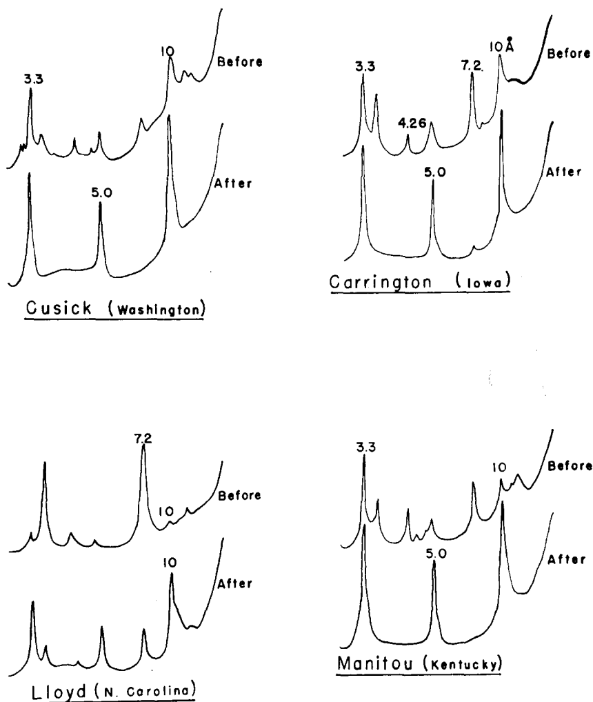
FIG. 1. Effect of the reaction of soil clays with the "F solution" for 24 hr as indicated by X-ray diffraction patterns of NH 4 -saturated samples heated at 110°C.
