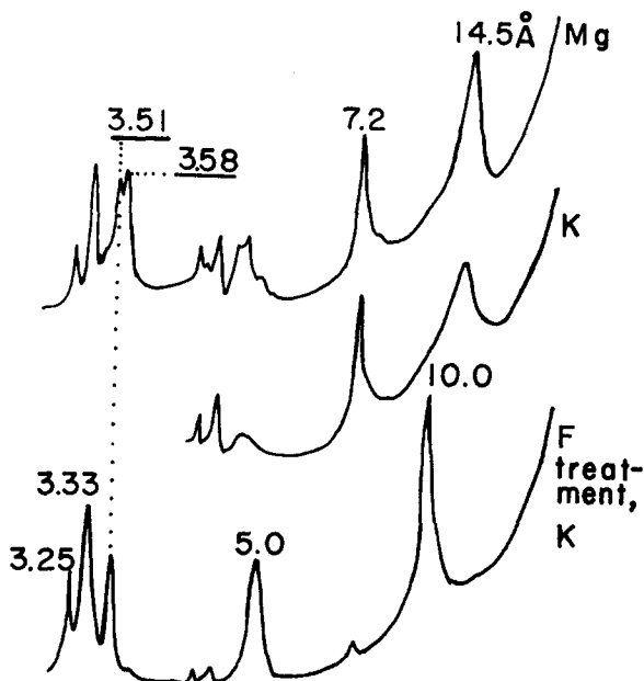
FIGURE 3.—Concentration of anatase in a Red Bay soil clay by a 24-hr reaction with the fluoride solution as indicated by X-ray diffraction patterns. The 3.51 Å peak is attributed to anatase.
