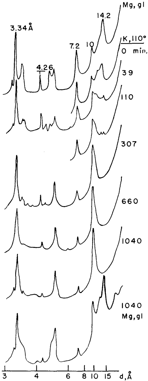
FIGURE 2.—Effect of reaction time of “F solution” on 2-0.2 μ fraction from a Matapeake B2 soil; also expansion of final product on Mg saturation.
