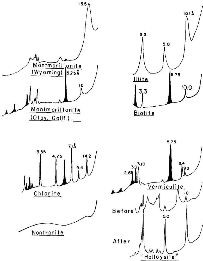
FIGURE 4.—Effect of the reaction of specimen minerals of clay size with the "F solution" for 24 hr as indicated by X-ray diffraction patterns of \text{NH}_4 -saturated samples. The reaction product, \text{MgNH}_4\text{AlF}_6 , is identified by "solid" peaks.
